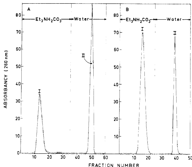
FIGURE 2: Column chromatographic separation of mononucleotides on borate gel. A mixture of the four standard ribonucleoside 5'-monophosphates (340 A_{260} units) and of the four deoxyribonucleoside 5'-monophosphates (190 A_{260} units) was applied in A. In B, a mixture of 16 mg of ribocytidine 5'-phosphate and 13 mg of riboadenosine 2'(3')-phosphate was chromatographed. Fractions of 1.3 ml were collected every 4 min from 25 cm \times 1 cm columns. The elution buffers are indicated by the arrows. By paper chromatographic (A) or spectral (B) analysis, material from the peaks was identified as a mixture of the four deoxyribonucleoside 5'-monophosphates (AI), a mixture of the four ribonucleoside 5'-phosphates (AII), riboadenosine 2'(3')-phosphate (BI), and ribocytidine 5'-phosphate (BII).
