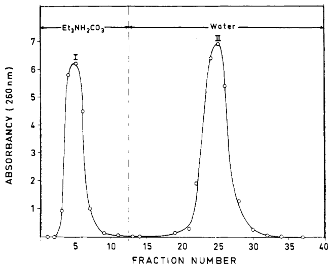
FIGURE 3: Column chromatographic separation of p(dT)_3 from p(dT)_4 -rU on borate gel. 200 A_{260} units from peak N-O of Figure 1 after removal of the solvent were dissolved in 1.5 ml of 1 M Et_3NH_2CO_3 and applied to the borate gel column (15 cm \times 1.5 cm). Elution was carried out with the buffers indicated by the arrows. Fractions of 4.5 ml were collected every 2–3 min.
