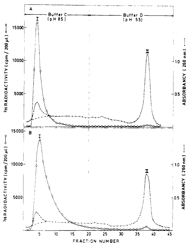
FIGURE 6: Purification of E. coli aminoacyl-tRNA by column chromatography on borate gels. (A) Separation of a tRNA mixture containing 674 pmol of [ ^3\text{H} ]glutamyl-tRNA (1.6%) in a total of 26.3 A_{260} units of tRNA; (B) separation of a tRNA mixture containing 1030 pmol of [ ^3\text{H} ]lysyl-tRNA (2.4%) in a total of 27.9 A_{260} units of tRNA. Elution buffers were applied as indicated by the arrows. Fractions of 4.6-ml volume were collected every 5 min in tubes containing 200 \mu\text{l} of 1 M sodium acetate, pH 4.5, in order to neutralize the eluent immediately. Aliquots of 200 \mu\text{l} were assayed for acid-insoluble radioactivity (O). Absorbancy of the individual fractions was followed at 260 nm (+); the absorbancy background of the elution buffer alone (---) is not subtracted in the figures.
